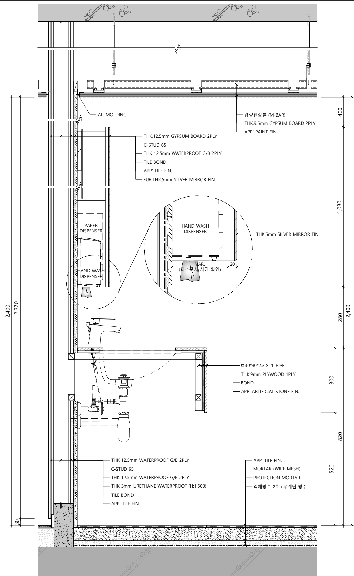
2 WALL SECTION-2
