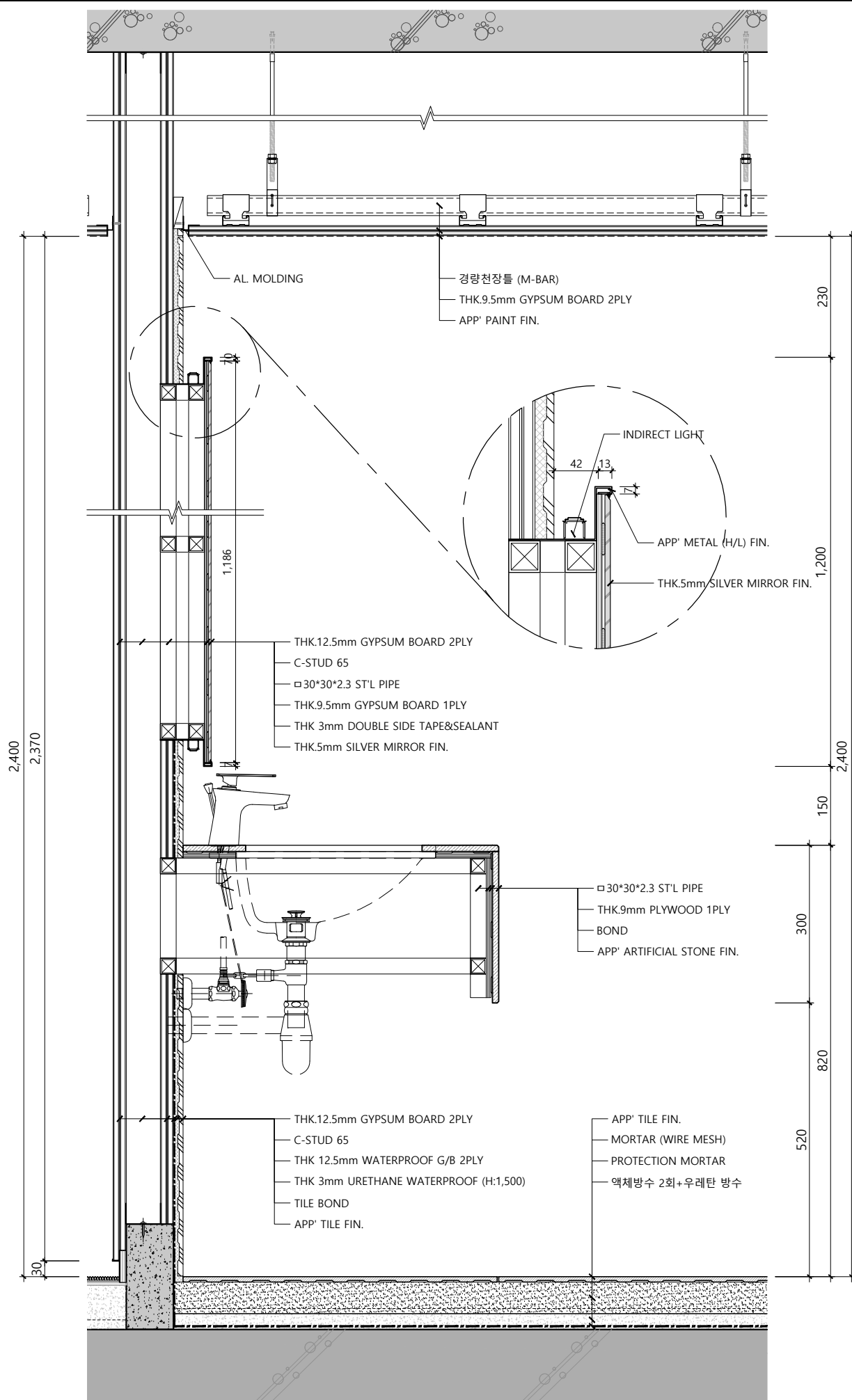
WALL SECTION-1
